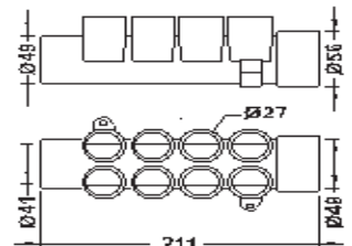
8 Port Water Manifold
