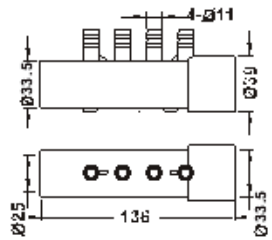
4 Port Air Barb Manifold
