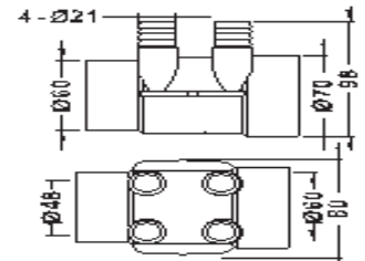
4 Port Water Barb Manifold
