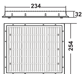
Square Main Drain(s)
