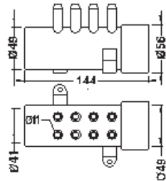
8 Port Air Manifold
