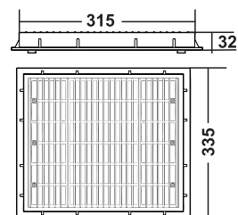
Square Main Drain(L)
